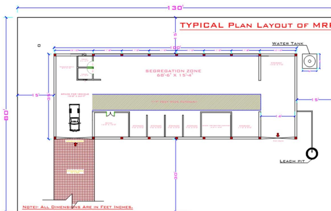
Figure 31: Layout Design of MRF
